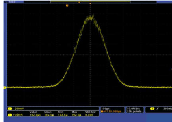
Typical Autocorrelation Trace
